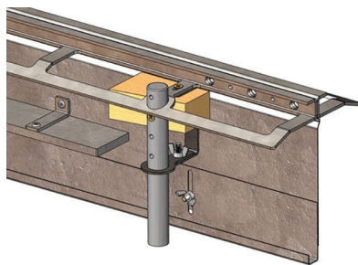
Beast Armored Joint Installation with Stake
