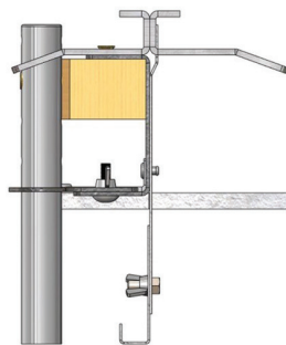
Pre-pour Condition - Both Sides of Beast Armored Joint
