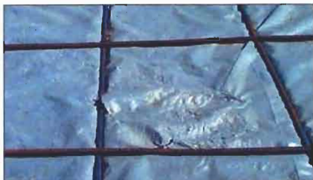
A thicker vapor barrier is required where there will be equipment traffic or with angular base materials. Note the example of torn 6-mil poly.
