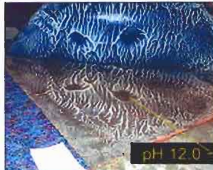
High moisture levels in the concrete cause soluble alkalis to enter into solution, raising the pH and leading to adhesive breakdown.
